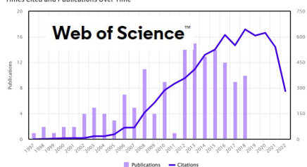
Times Cited and Publications Over Time
